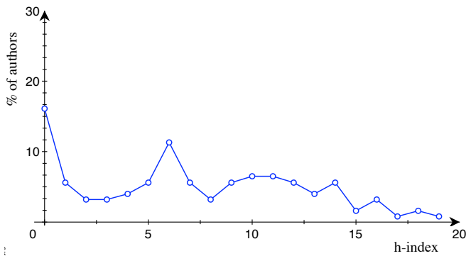
Figure 2. Percentage of authors with a given h -index
